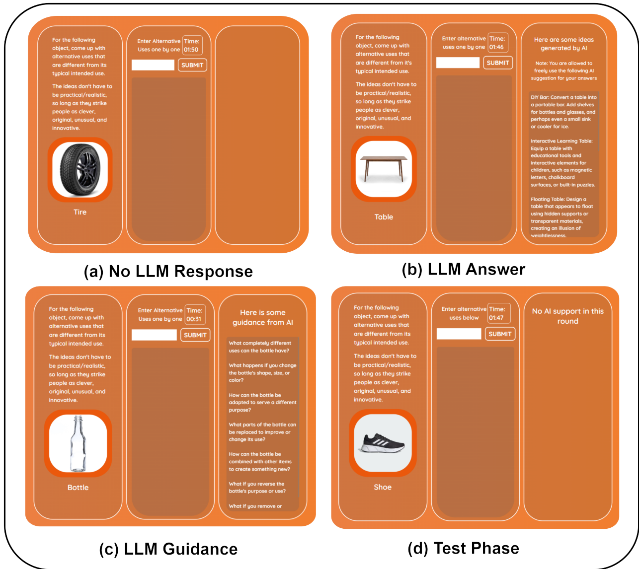
Figure 3: Interface used in the divergent thinking experiment across all 3 exposure round conditions and test rounds.
